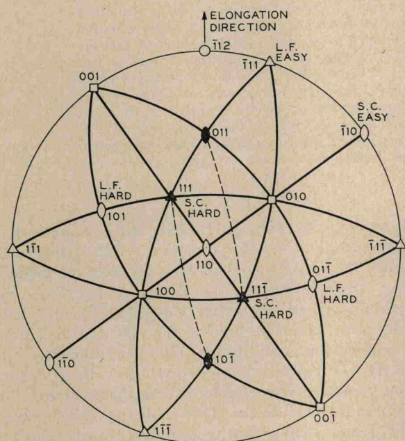
FIG. 1. (110) stereographic projection of a cubic crystal. During (110) [\bar{1}12] plane-strain compression, (111) [10\bar{1}] and (111) [011] slip systems become active. In L.F. deformation, [0\bar{1}\bar{1}] and [10\bar{1}] , which are perpendicular to the slip directions [011] and [10\bar{1}] , respectively, become hard axes, resulting in [\bar{1}11] being the easy axis. In S.C. deformation, the slip plane normals [111] and [11\bar{1}] are hard axes, leading to [\bar{1}10] as the easy axis.
